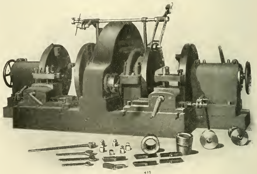
LATEST POND STEEL TIERED CAR WHEEL LATHE.
